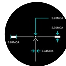
Winchester® Supreme® Post w/ Dot Reticle
