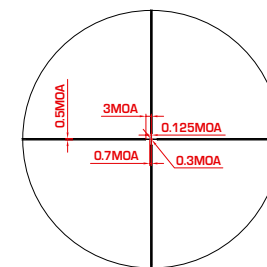
Winchester® Supreme® Illuminated Reticle 6-18x50
